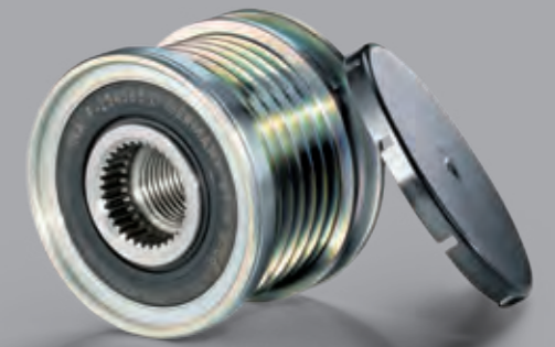
Overrunning alternator pulley
